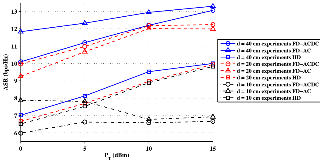
Fig. 10. Experiment results showing an increase in the achievable sum rate as a function of the transmission power for a full-duplex two-way system using the same transmission power P_T at both nodes. The figure also shows results for half-duplex experiments where the transmit power per antenna was set equal to P_T . Hence, for each P_T value, the systems compared have the same average transmitted power per node. Each data point corresponds to two 800 frame experiments whose results were averaged to obtain one data point.
