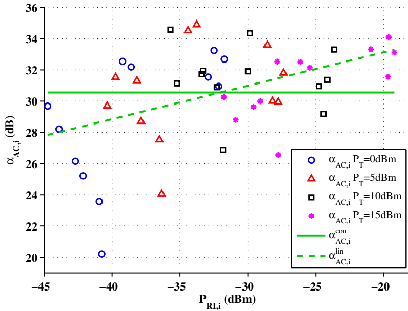
(a) Results for active analog cancellation. The constant fit is equal to \alpha_{AC,i}^{con} = 30.55 dB and the linear fit is equal to \alpha_{AC,i}^{lin} = \lambda_{AC}P_{RI,i} + \beta_{AC} where \lambda_{AC} = 0.21 dB/dBm and \beta_{AC} = 37.42 dB.
