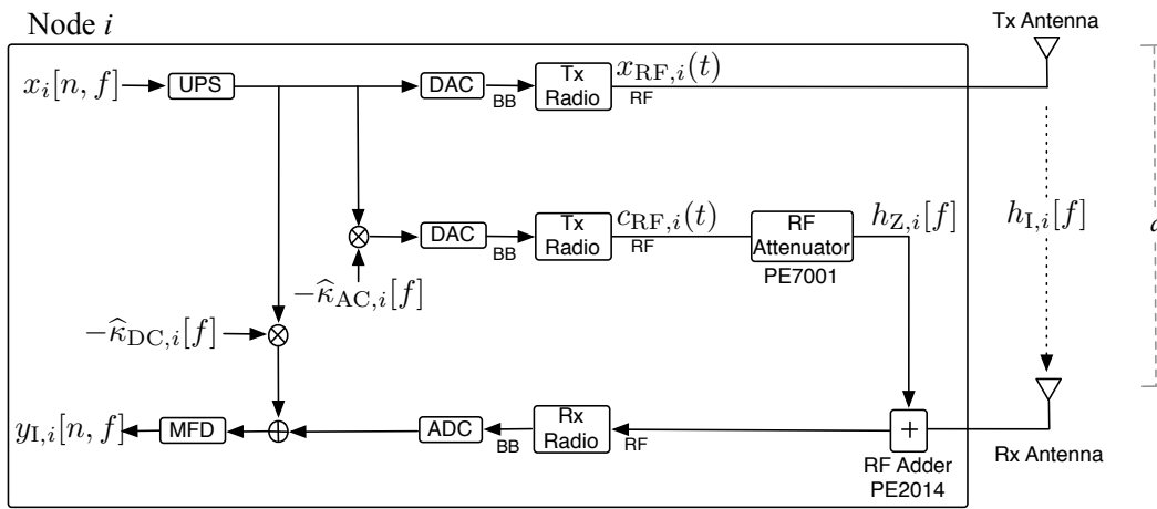
Fig. 1. Block diagram of a full-duplex node.
