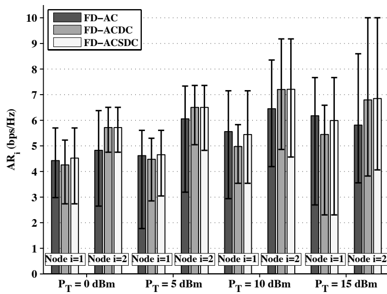
Fig. 11. Experiment results showing the effect of different cancellation schemes on the achievable rate per node of a full-duplex two-way system using the same transmission power P_T at both nodes. Results correspond to d = 20 cm and a distance between Node 1 and Node 2 equal to 8.5 m. Each bar corresponds to results from two 800 frame experiments.
