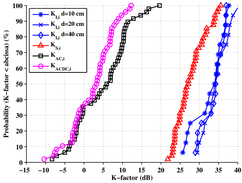
Fig. 7. CDF of K -factor. We aggregate K_{I,i} values computed for i = 1, 2 and different values of P_T to obtain the CDF of K_{I,i} for a fixed d . We obtained the CDF of K_{AC,i} and K_{ACDC,i} by aggregating the K -factors computed for i = 1, 2 for different values of d and P_T .
