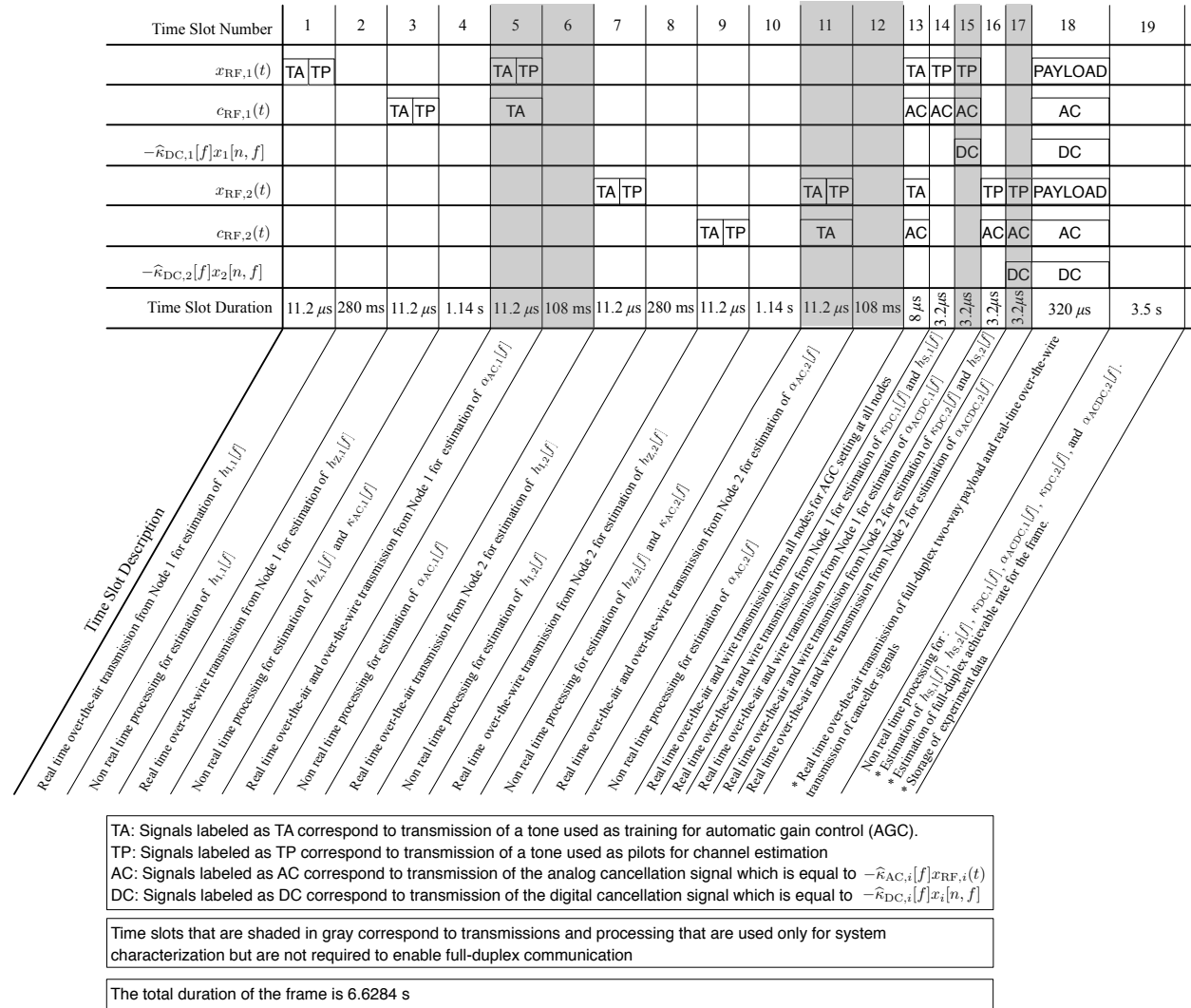
Fig. 2. Time diagram for a full-duplex frame.
