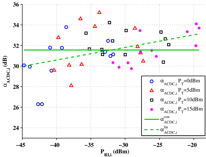
(b) Results for combined active analog and active digital cancellation. The constant fit is equal to \alpha_{ACDC,i}^{con} = 31.56 dB and the linear fit is equal to \alpha_{ACDC,i}^{lin} = \lambda_{ACDC}P_{RI,i} + \beta_{ACDC} where \lambda_{ACDC} = 0.12 dB/dBm and \beta_{ACDC} = 35.49 dB.
