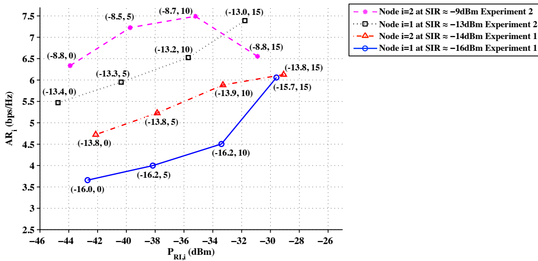
Fig. 9. Experiment results showing the achievable rate for transmission to Node i as a function of the average received self-interference power at Node i for an approximately constant value of SIR_{AS,i} . All the results correspond to a full-duplex system with active analog cancellation, active digital cancellation, a distance d = 40 cm between self-interfering antennas, and a distance of 8.5 m between Node 1 and Node 2. Both nodes used the same transmission power P_T and we were able to increase P_{RI,i} , while keeping SIR_{AS,i} constant, by increasing P_T . The exact values of SIR_{AS,i} and P_T for each data point are shown in parenthesis as a pair of values (SIR_{AS,i} \text{ (dB)}, P_T \text{ (dBm)}) next to each data point. Each data point corresponds to an 800 frame experiment and for each node we show two curves because we did the same 800 frame experiment twice. The second experiment was done a few days after the first experiment hence the conditions surrounding the setup were not exactly the same for the two experiments (due movement of people in the laboratory) and this explains why the rates at a node are different between experiments.
