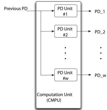
Fig. 6. Computation Unit (CMPU)
